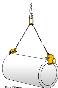
For Pipes
