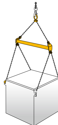
For Balance Beams/Distance Bars
